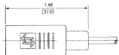
In-Line Receptacle
